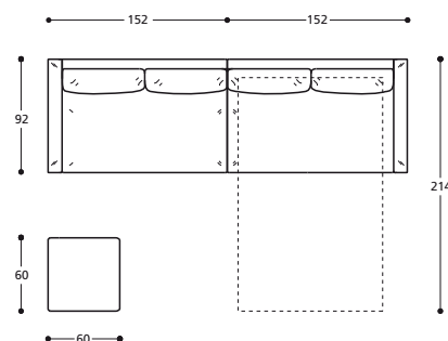
1 X ART. 8489 HOCKER 60X60 1 X ART. 8476 ELEMENT 152 1 X ART. 8472 BETTELEMENT 152
